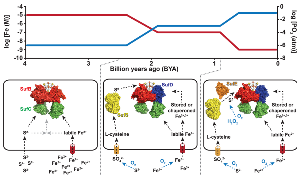
Figure 1. Model of core Suf pathway evolution in response to increasing oxygen concentrations in the biosphere. In the top graph, iron (red) and oxygen (blue) concentrations refer to those in seawater as adapted from published estimates. 1 The bottom panels show the addition of biogenesis components to the core SufBC scaffold complex in response to decreased iron bioavailability (SufD), altered sulfur metabolism (SufS), and oxidation of sulfur transfer intermediates (SufE). Surface representation structures are of SufB (red), SufC (green), SufD (blue), SufS homodimer (yellow), and SufE (orange). The model shows SufBC performing its proposed role as an Fe–S cluster scaffold. A proposed role for SufD in iron acquisition is also shown. SufS and SufE are shown mobilizing sulfide (as persulfide) from L-cysteine for cluster biogenesis in some species. See Table 1 for a summary of proposed Suf protein functions and the text for more details.
